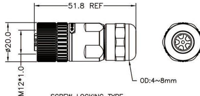
SCREW LOCKING TYPE
