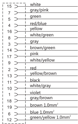
Circuit diagram/电路图
